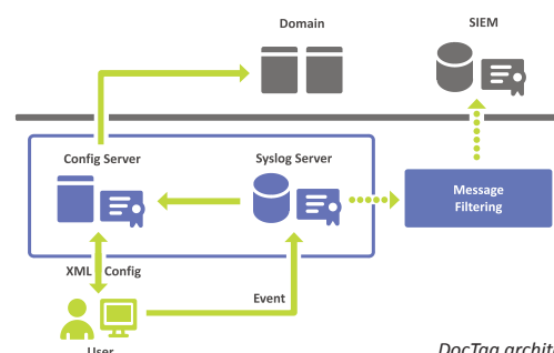
DocTag architecture
